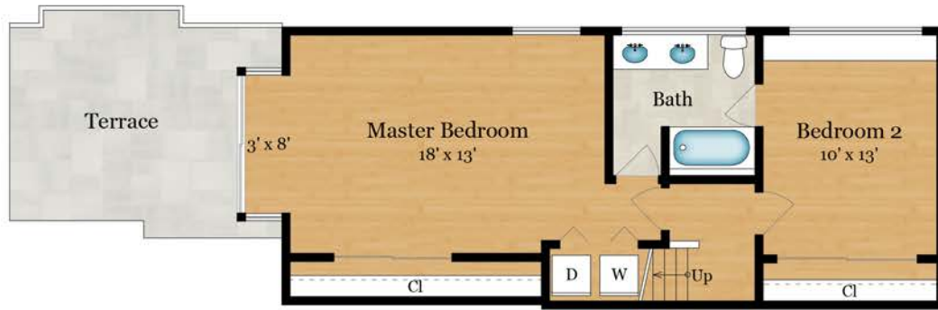
LOWER LEVEL 640 SQ FT
